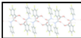
Fig. 3. Hydrogen bonding interactions (blue dotted lines; red dotted lines indicate hydrogen bonding continuation) in (I).
