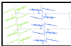
Fig. 4. A b -axis projection of the crystal packing in (I). The colour scheme is that used in Figure 2.
